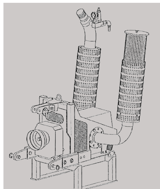
3-point hitch PTO driven air compressor
